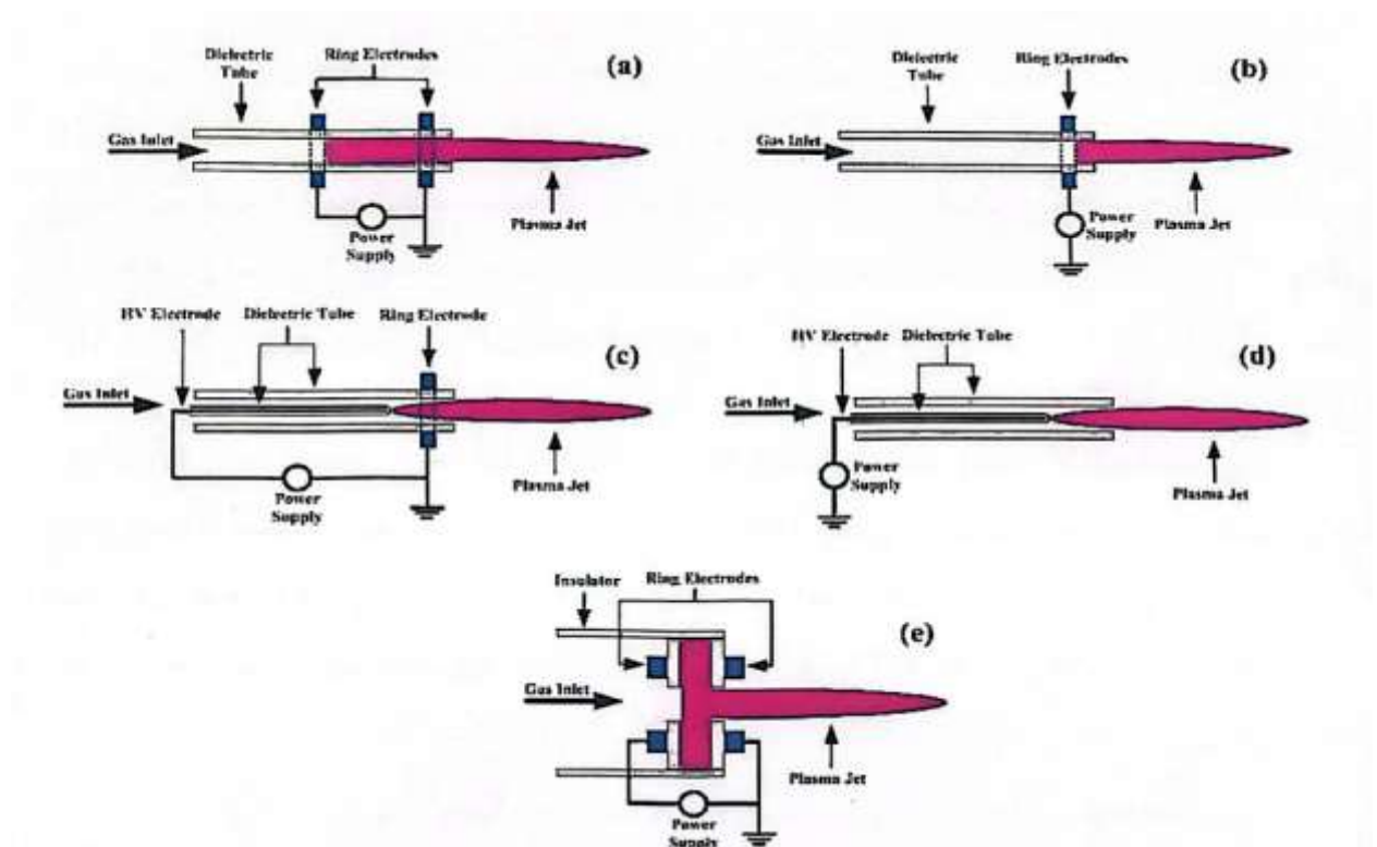
[Figure 3] Atmospheric Pressure Plasma Jets (APPJs) based on the DBD technology to produce cold plasma.
